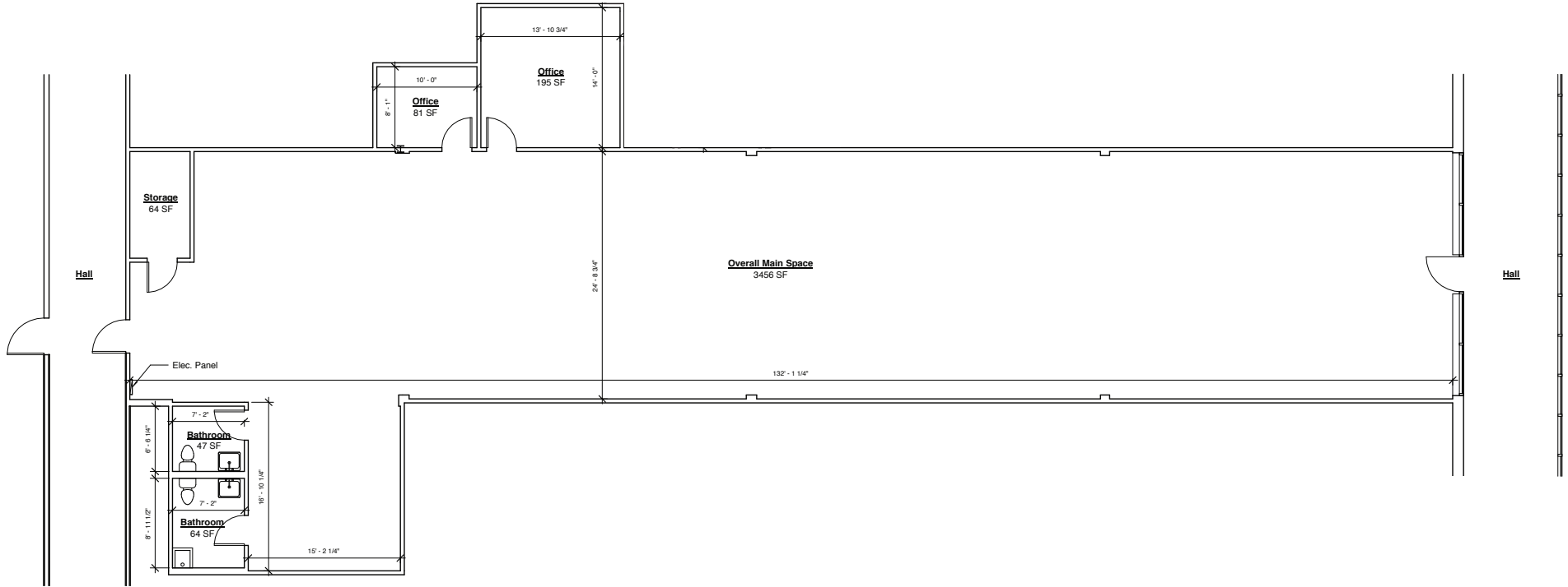
1 First Floor Plan Existing 3/16" = 1'-0"
